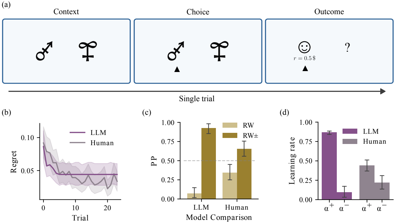
Figure 2. 2AFC task with partial feedback. (a) Presentation of a single trial. First, two slot machines, shown as symbols, are presented. After a choice is made, the outcome is shown. (b) Average performance of the LLM and humans measured in terms of regret. Performance improves over trials. (c) Model comparison of the Rescorla-Wagner (RW) model and the RW± model. For both the LLM (left) and human participants (right), RW± provides a better fit to the data, as indicated by the average posterior probability (PP). (d) Average learning rates of the RW± model for the LLM and human participants. Both agents show a stronger response to positive prediction errors than to negative prediction errors. Human participant data reproduced from (Lefebvre et al., 2017). Error bars and shaded areas and correspond to 95% CIs.
