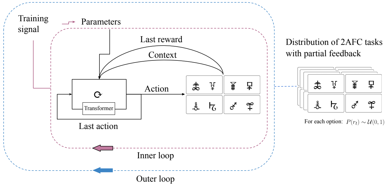
Figure 8. Schematic of the Meta-RL training for Task 1 highlighting the inner and outer training loops. The outer loop adjusts the weights of the Transformer in response to the learning experience. These weights shape the behavior of the Transformer in the inner loop as it interacts with 2AFC tasks (here Task 1). After each cycle of the outer loop, a new task is sampled where the probabilities for each option are sampled from a uniform distribution. Adapted from Botvinick et al. (2019).
