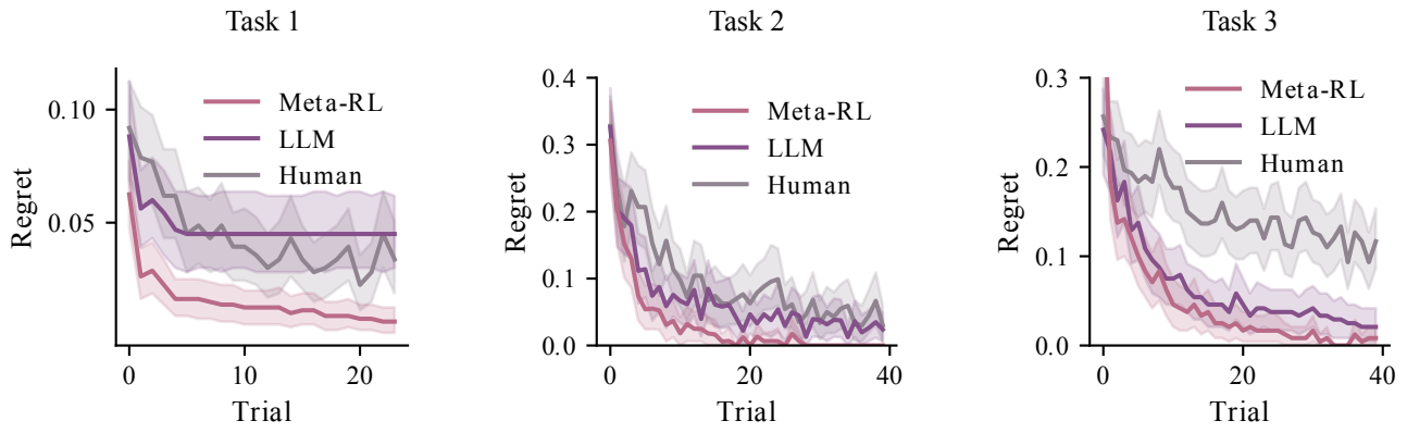
Figure 9. Average performance comparison of all three agents in terms of regret. In all tasks, the Meta-RL agent improves its performance over time fastest. Shaded areas correspond to 95% CIs.
