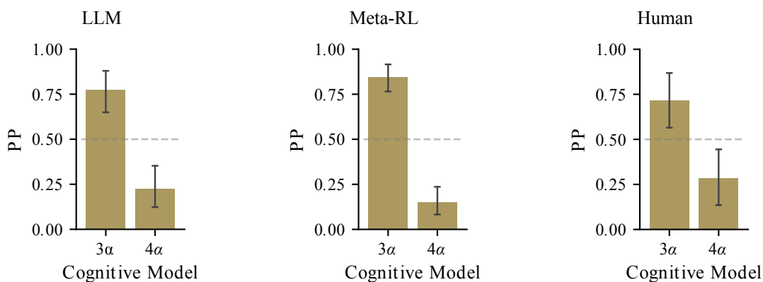
Figure 7. Model comparison for the agency condition for all agents. The 3\alpha model has the highest average posterior probabilities (PP). This indicates that information from forced-choice trials where no agency is involved are weighted symmetrically whereas the free-choices are weighted asymmetrically. Error bars correspond to 95% CIs.
